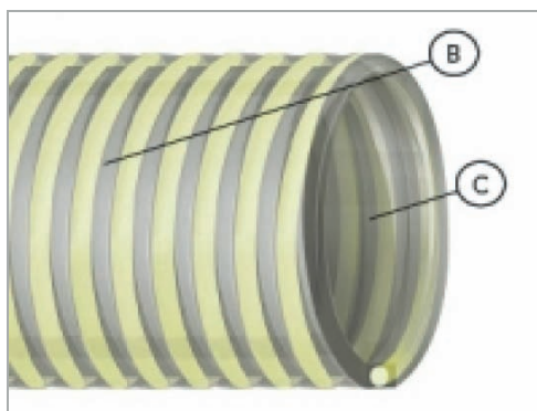
PVC wall (B) with inner ply food grade PU resistant to abrasion (C)
