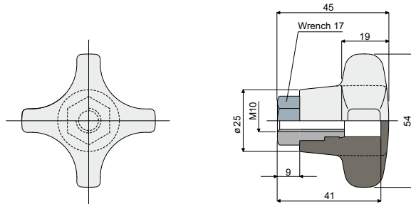
Knob for bracket Part. 247 (reinforced type)
