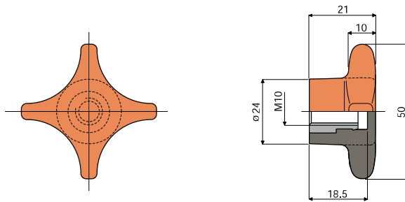
Knob for bracket Part. 313 (short type)
