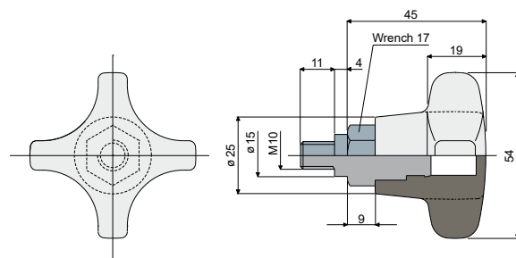
Knob for bracket Part. 248 (reinforced type)
