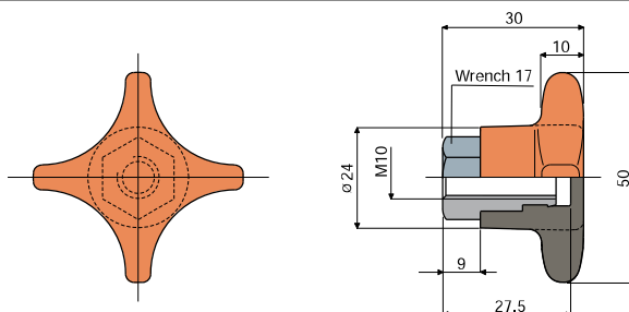
Knob for bracket Part. 314 (short type)
